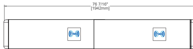
Double Charger Unit (Horizontal Only)
